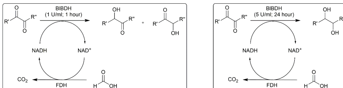
1: R'=R''=CH_3 2: R'=R''=CH_3 3: R'=CH_3 , R''=OH-CH_2-CH_3 4: R'=CH_3 , R''=O-CH_2-CH_3 5: R'=CH_3 , R''=CH_2-CH_3 6: R'=CH_3 , R''=CH_2-(CH_2)_2 7: R'=R''=CH_2-CH_3 8: R'=CH_3 , R''=(CH_2)_3-CH_3 9: R'=R''=CH_2-CH_3 10: R'=CH_3 , R''=(CH_2)_2-CH_3 11: R'=Ph , R''=CH_3 12: R'=Ph , R''=CH_3 13: R'=Ph-(F)_3 , R''=CH_3 14: R'=Ph-(F)_3 , R''=CH_2-CH_3 15: R'=Ph , R''=CH_3
